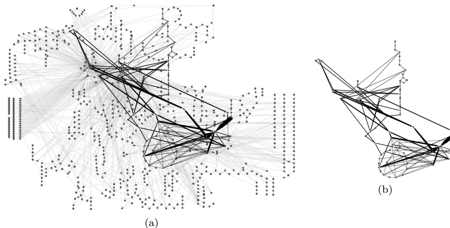
Fig. 3. Filtering and subnetwork features. For the analysis of flux distributions in medium to large-scale networks limitation of network views based on selected attributes is crucial. (a) Flux distribution in the full network (b) flux subnetwork with much lower complexity. Flux distribution is FASIMU FBA result in a reconstructed human hepatocyte network (supplementary information). Flux Minimization [4] was used as objective function in the analysis of glucose formation from oxalacetate. Manually generated Layout, linear (linear flux edge weight) mapping function. Subnetwork is flux subnetwork and consists of edges and nodes with non-zero flux. FluxViz subnetworks can be generated based on arbitrary network attributes like flux values or node localization.
